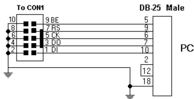
ISP Download cable
