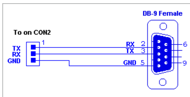
Fig. 4 RS232 cable
